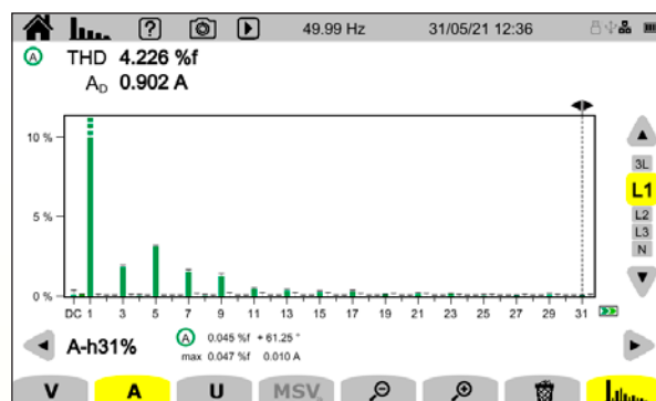
It is very simple to measure harmonics and interharmonics with the CA 8345, which is very easy to use as an analytical tool.
